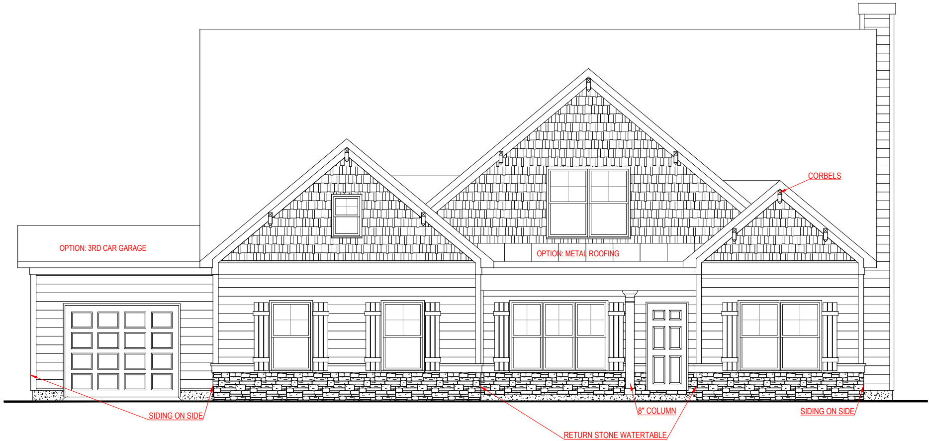
FRONT ELEVATION - B VERSION
