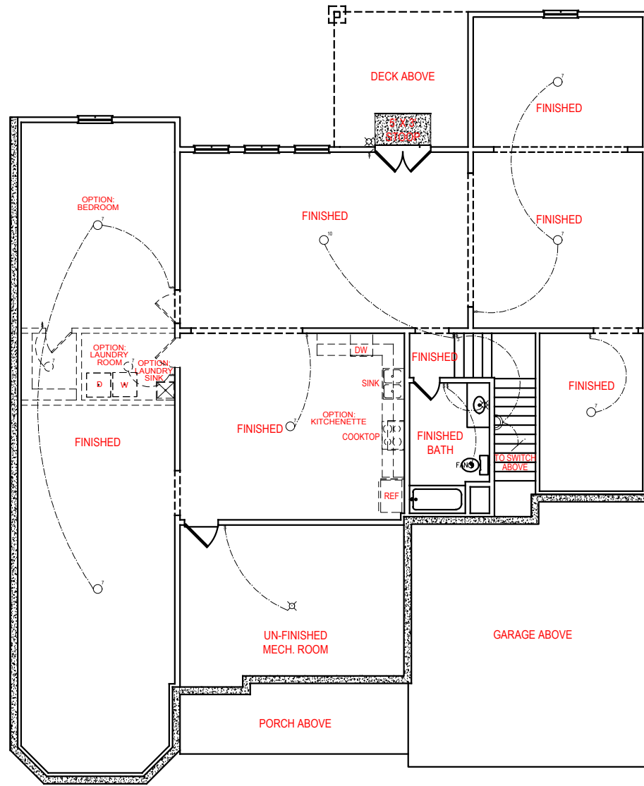
OPTION THREE: FINISHED BASEMENT ADDS 2,340 SQ. FT.
